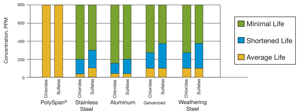
Chloride & Sulfate Concentration Guidelines for Pipeline Life
